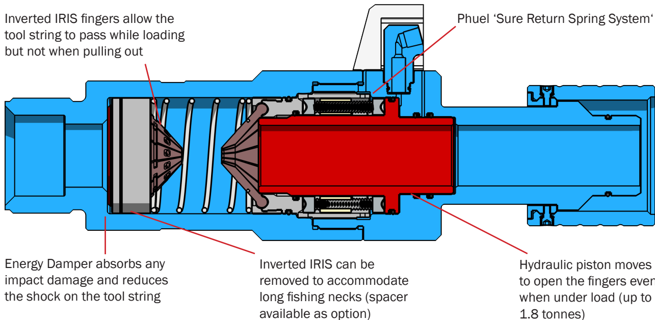
Slickline Stack
