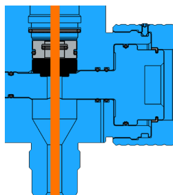
Unactivated Position
